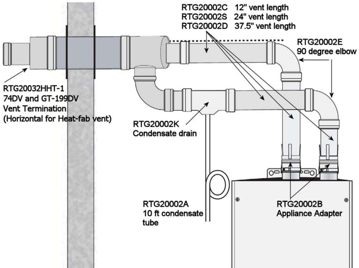
74DV and GT-199DV Horizontal Vent Termination (Heat-fab vent)
